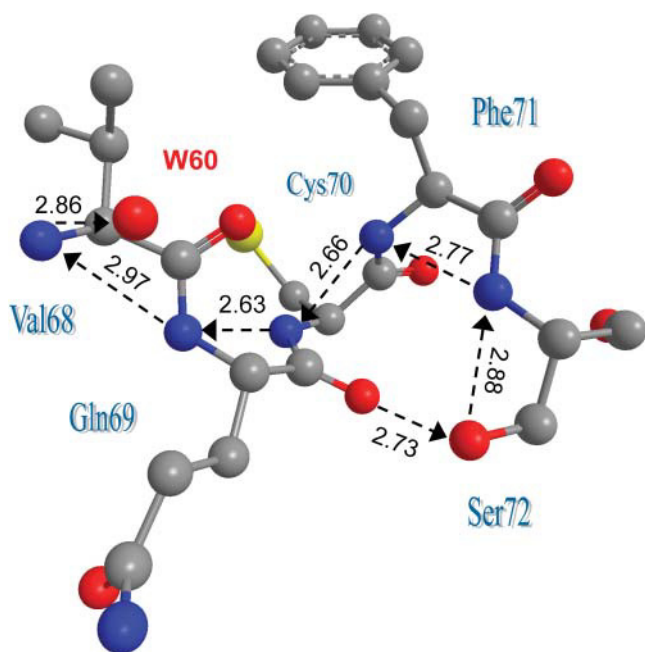
FIGURE 8 A bb-nitrogen wire could serve as an alternative to W255 in bridging the gap between Ser-72 and W60. The nitrogens also couple to the bb-carbonyls of Val-68 and Gln-69, allowing several shortcuts to be taken. Coordinates from PDB file 1GFL.
