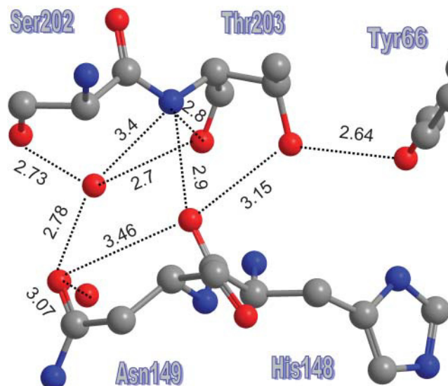
FIGURE 4 A more extended exit channel may continue from the bb-carbonyl of His-148 along various solvent-protruding side chains or surface water molecules. Interatom distances in angstroms. Color codes as in Fig. 2. Coordinates from PDB file 1Q4A.
